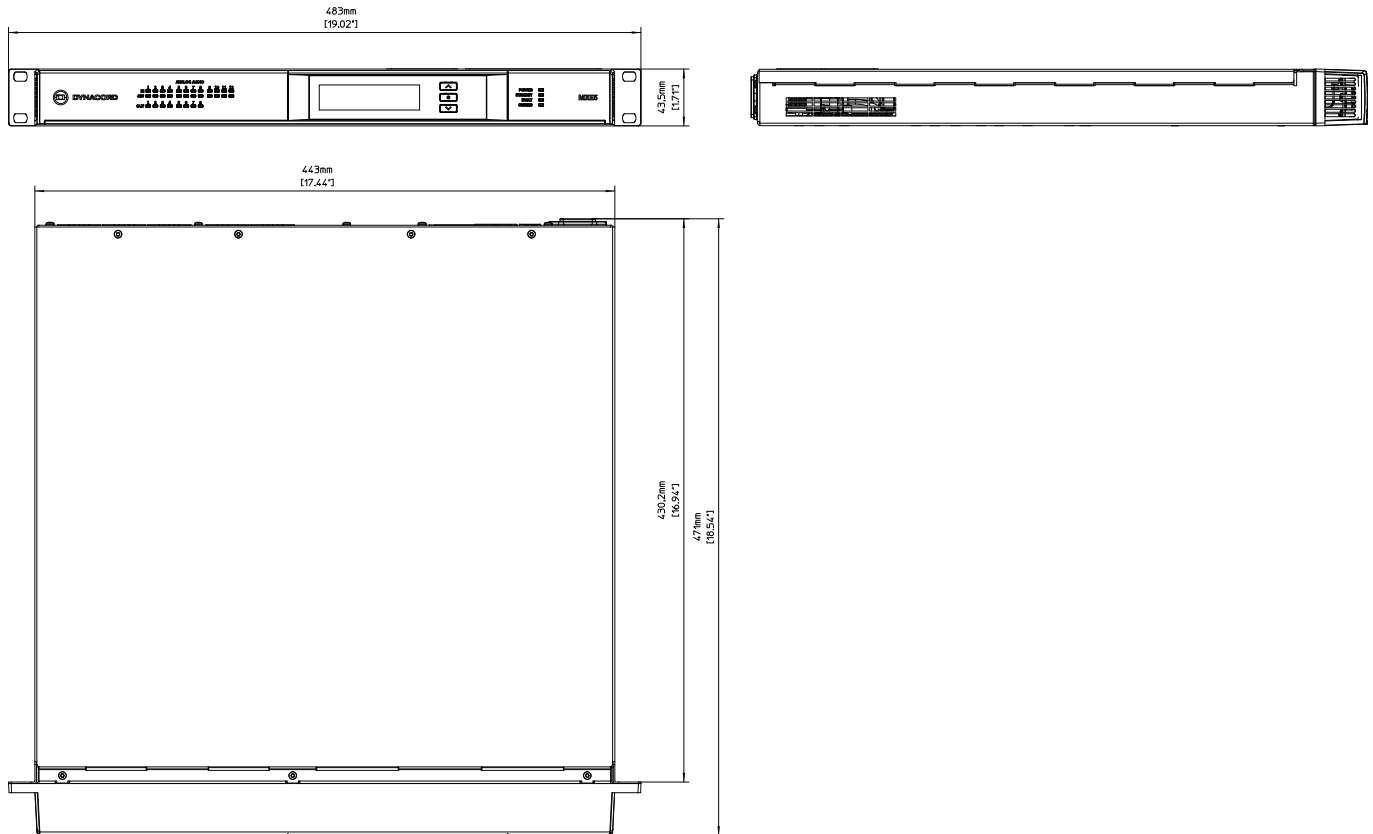
Dimensions: MXE5
