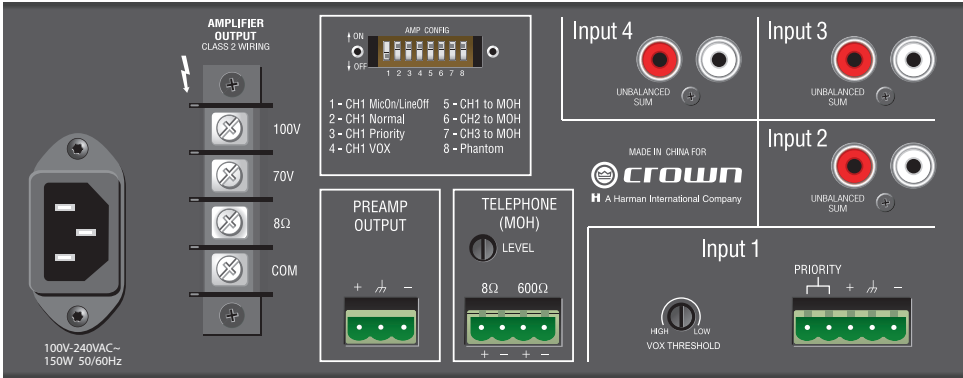
160MA back panel
