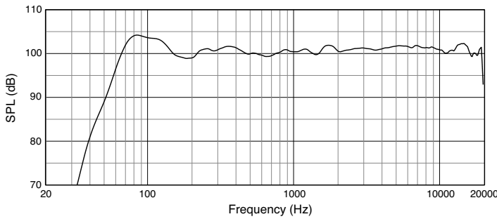
Frequency Response (Monitor)
