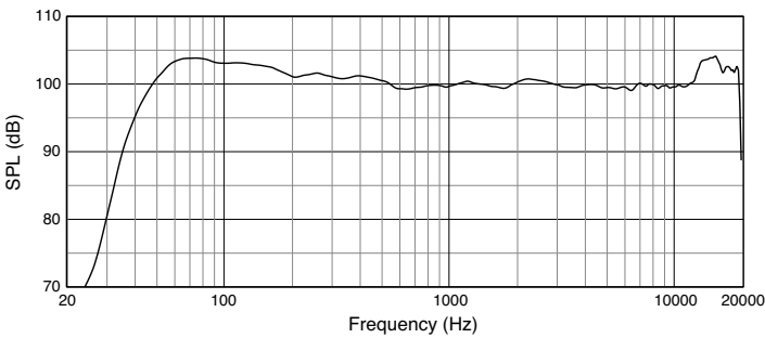
Frequency Response (Speech)
