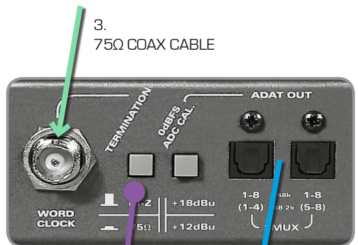
1. MASTER CLOCK SOURCE BNC OUTPUT to ASP800 WORD CLOCK INPUT
