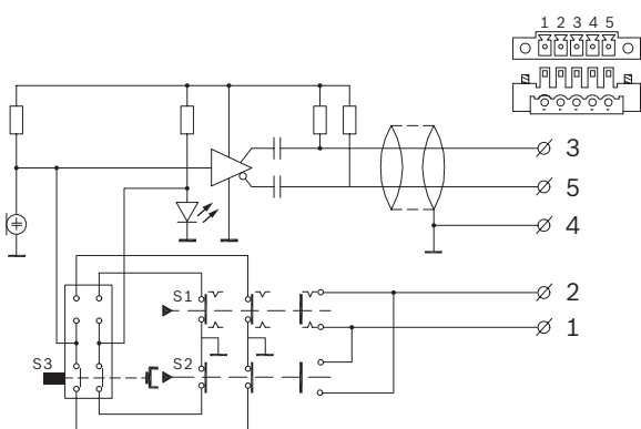
Circuit diagram
