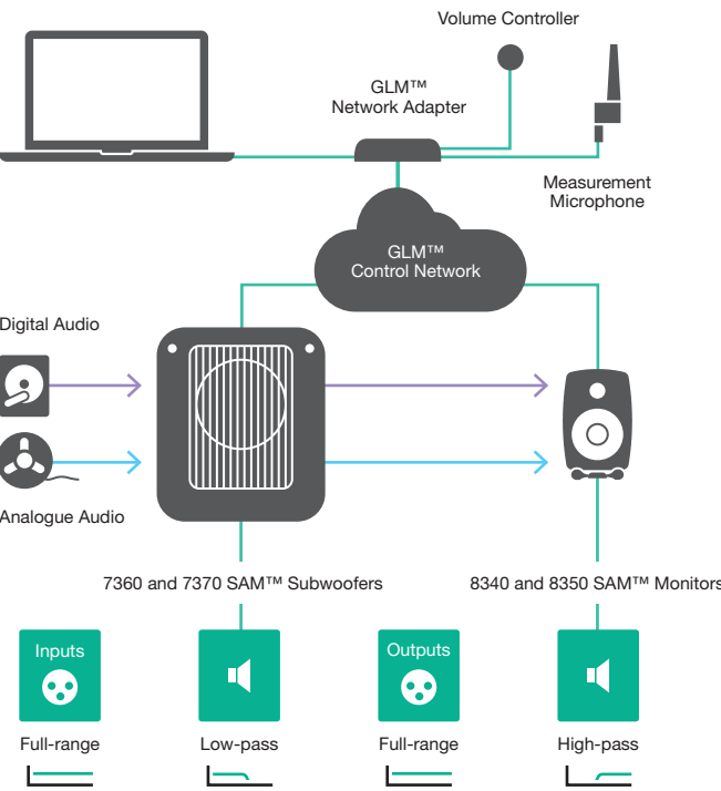
SAM™ System's basic connections and functionalities
