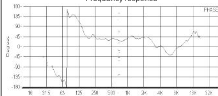
Phase response
