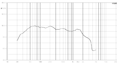
Frequency response
