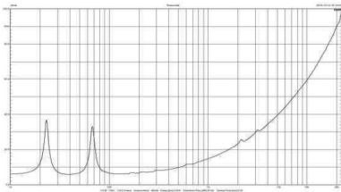
Impedance
