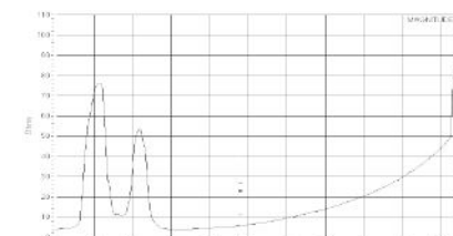
Impedance
