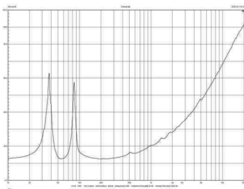
LF Impedance
