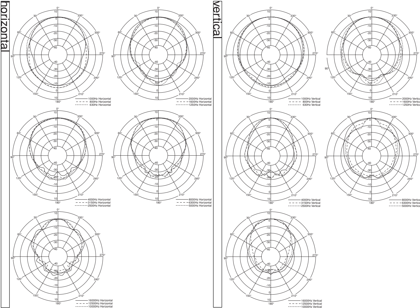
Polar Response
