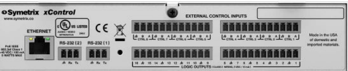
xControl Part Number 80-0089
