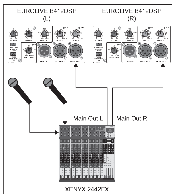
Fig. 4.2: Connecting a mixing console
