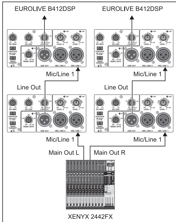
Fig. 4.3: Linking several B412DSP speakers
