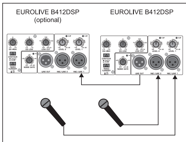
Fig. 4.1: Connecting microphones
