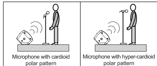
Fig. 3.3: The B412DSP as a monitor loudspeaker
