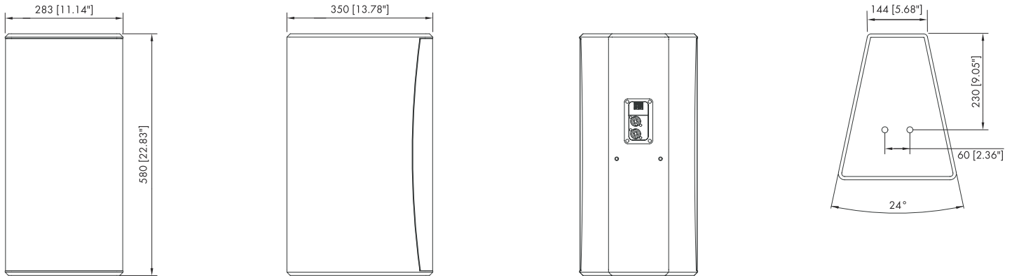
10S-D cabinet dimensions in mm [inch]
