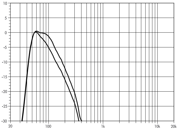
Fig. 6: 125-SUB frequency response, standard and 100 Hz modes
