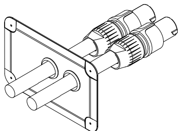
Fig. 5: NL4 cable connection with cover plate [1]
