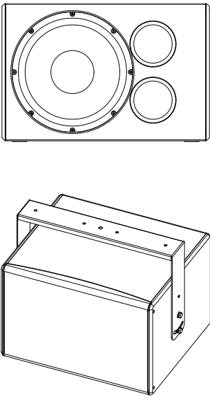
Fig. 1: 12S-SUB loudspeaker Rigging example: 12S-SUB ceiling mounted with Z5412 Horizontal bracket 12S-SUB.
