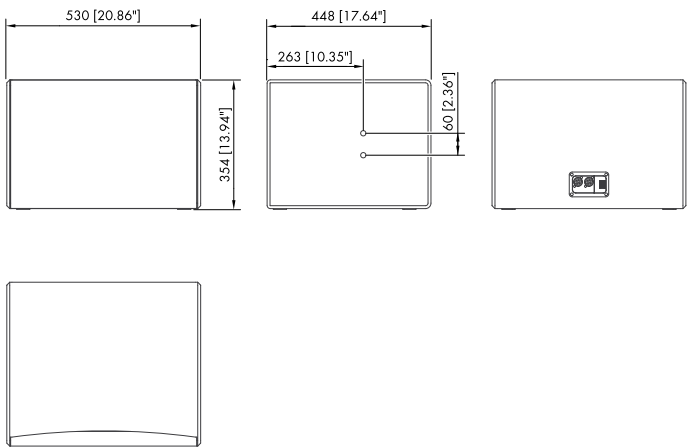
Fig. 7: 125-SUB cabinet dimensions in mm [inch]
