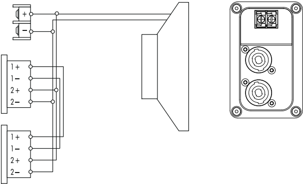
Fig. 2: Connector wiring
