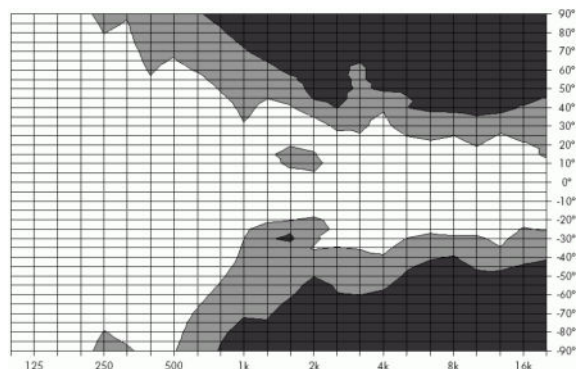
Fig. 13: Isobar diagram vertical
