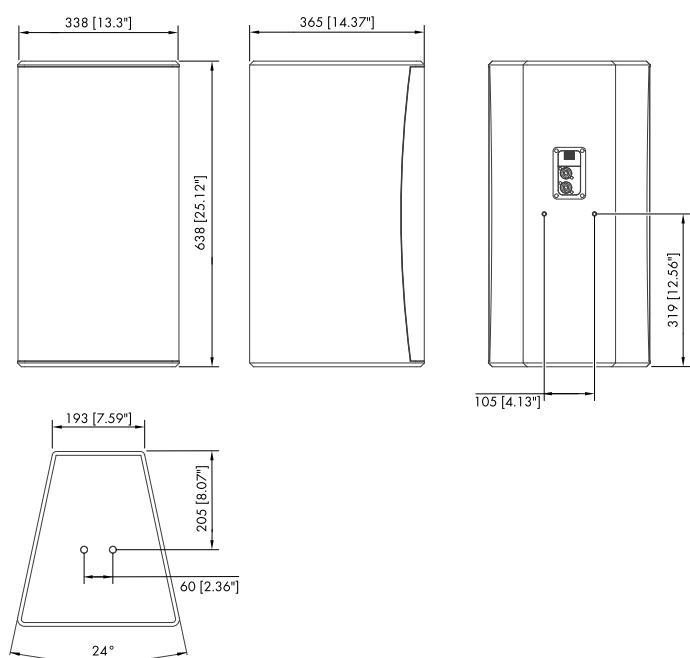
Fig. 18: 12S/12S-D cabinet dimensions in mm [inch]
