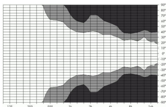
Fig. 15: Isobar diagram vertical
