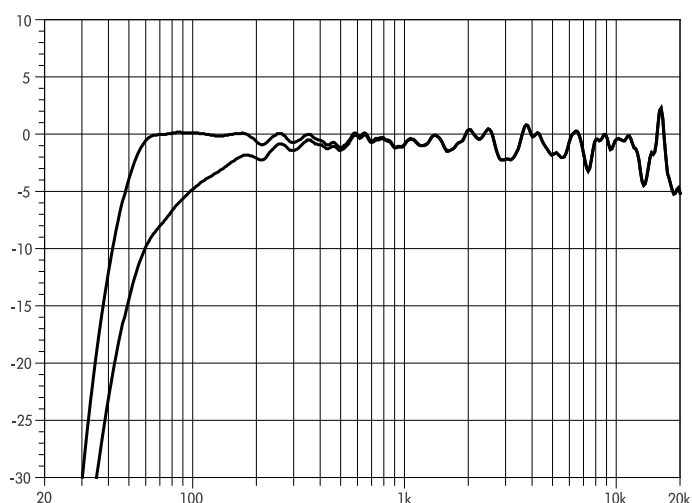
Fig. 17: 12S-D frequency response, standard and CUT modes
