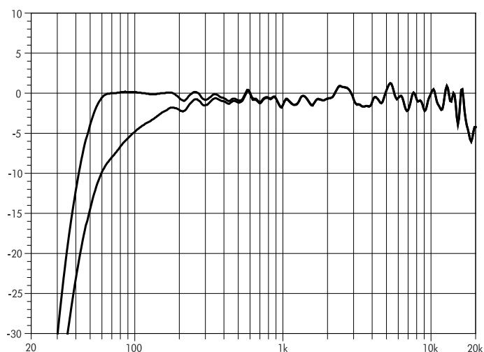
Fig. 16: 12S frequency response, standard and CUT modes
