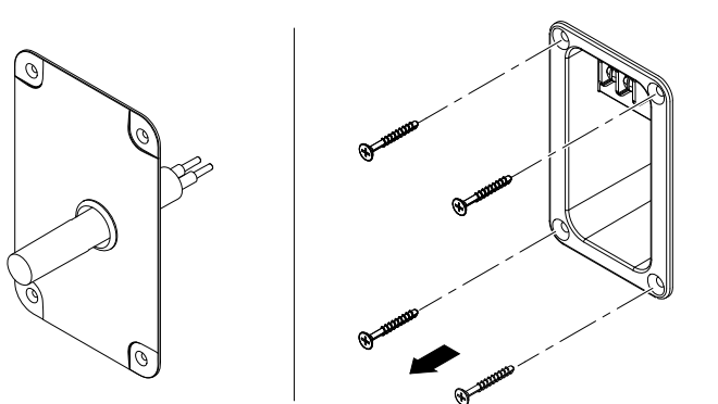
Fig. 4: Installing the fixed cable connection
