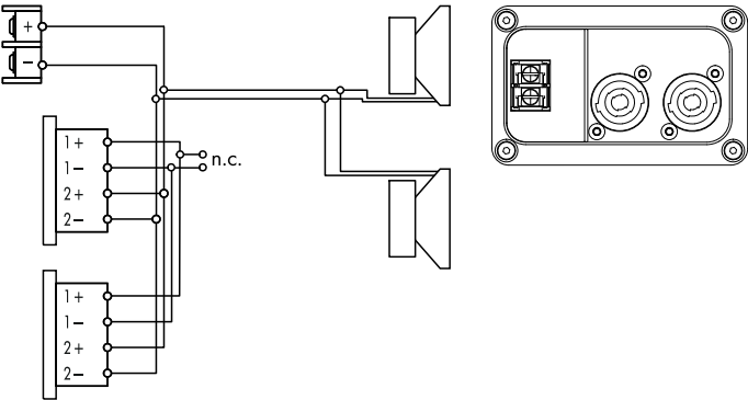
Connector wiring
