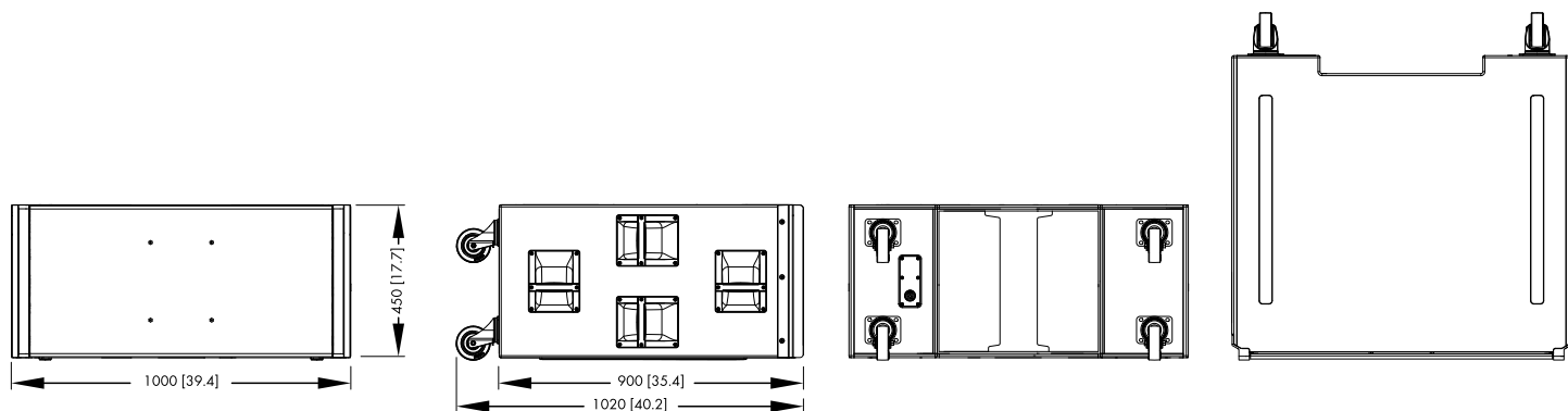
KSL-GSUB cabinet dimensions in mm [inch]
