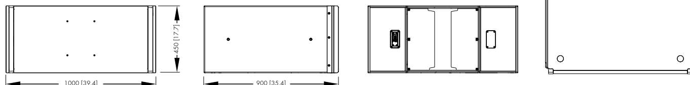
KSLi-GSUB cabinet dimensions in mm [inch]
