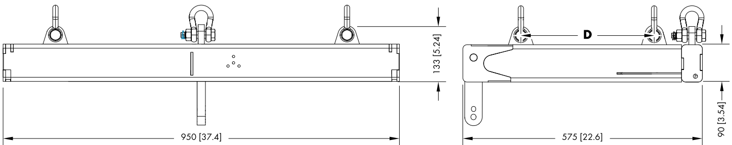
Z5743 KSLi-TOP Mounting frame dimensions in mm [inch]
