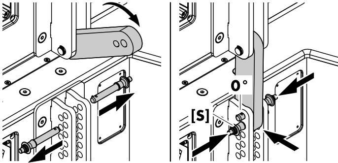
Set splay angle (e.g. 0°)
