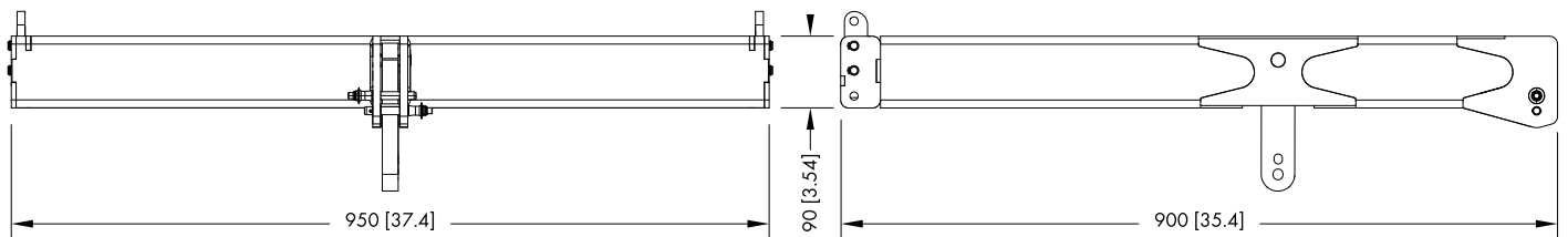
Z5745 KS Li-SUB Mounting adapter dimensions in mm [inch]
