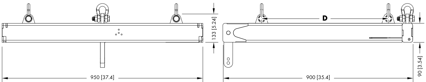
Z5744 KSLi-SUB Mounting frame dimensions in mm [inch]
