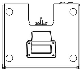
T-SUB cabinet dimensions in mm [inch]
