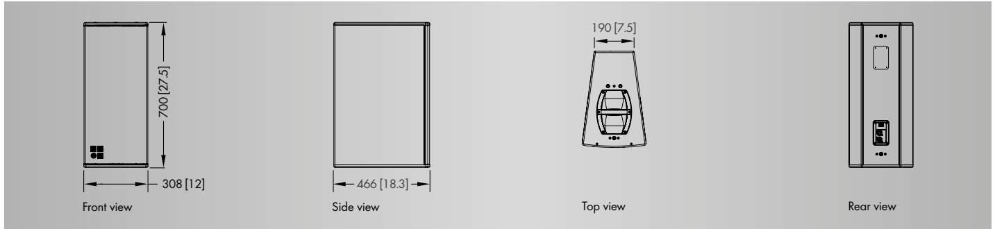
V10P cabinet dimensions in mm [inch]
