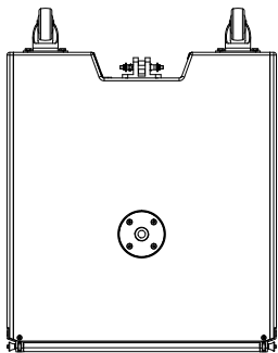
Y-SUB cabinet dimensions in mm [inch]
