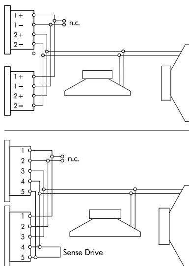
NLT4 F/M/NL4 M and EP5 connector wiring
