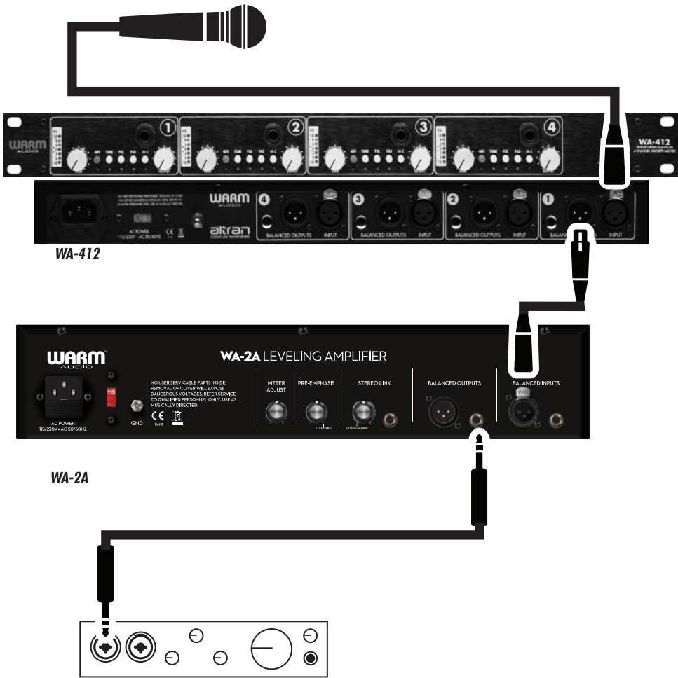
Recording interface
