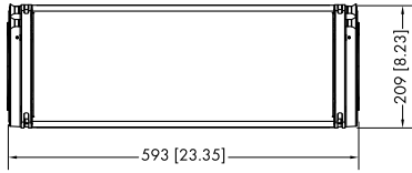
CCL8 cabinet dimensions in mm [inch]
